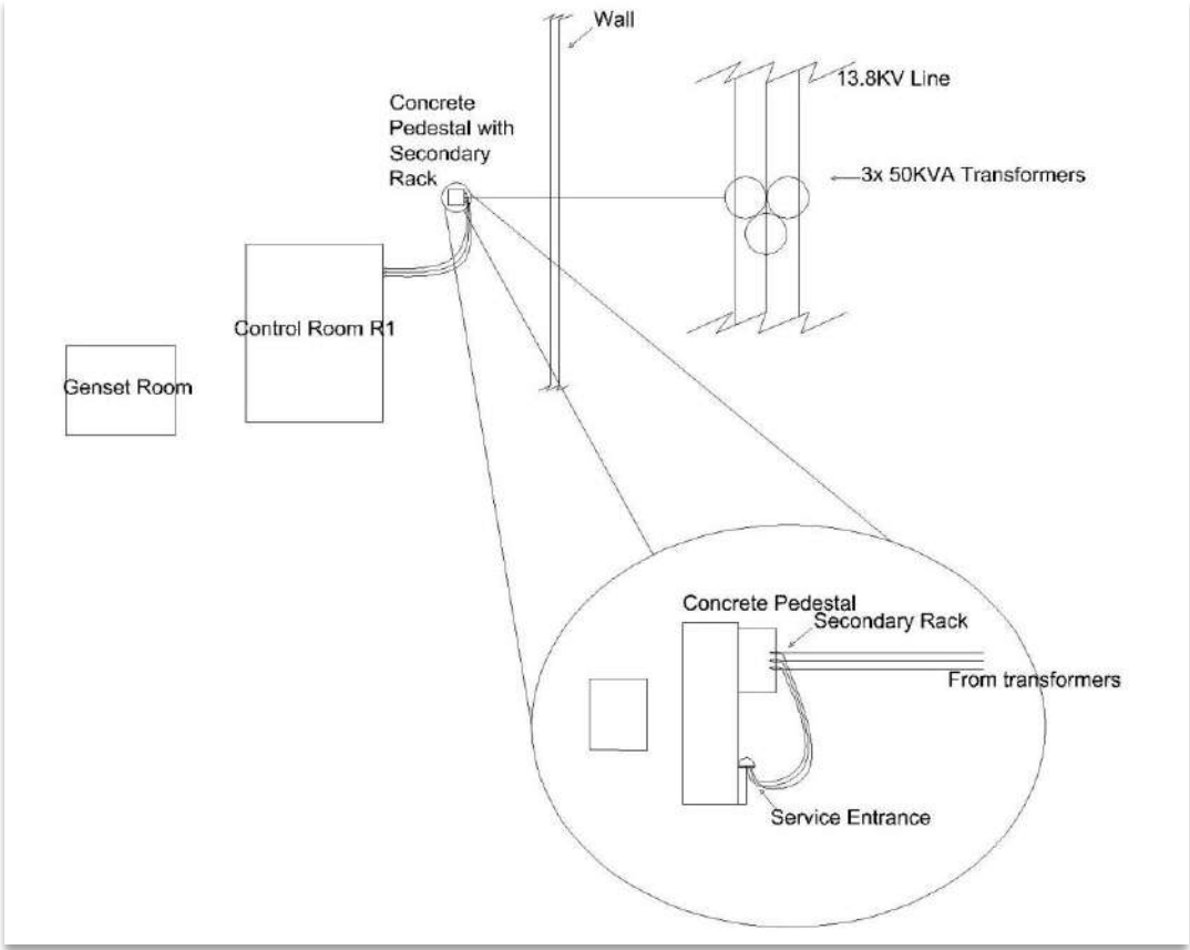
Drawing C: Service Conductors supported by 3-spool Secondary Rack
