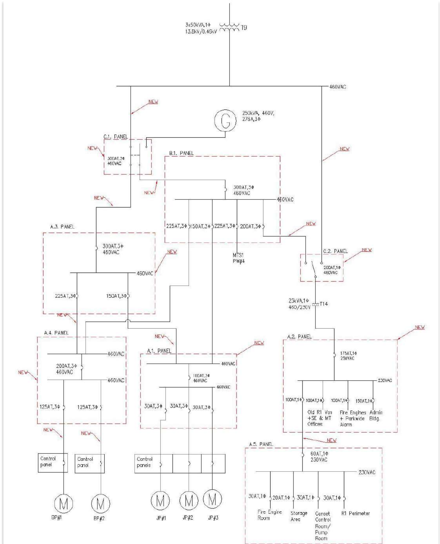
Drawing B: Proposed Electrical System Single Line Diagram (SLD)
