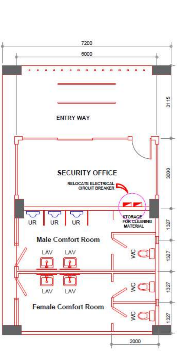
PROPOSE NEW LAYOUT PLAN
