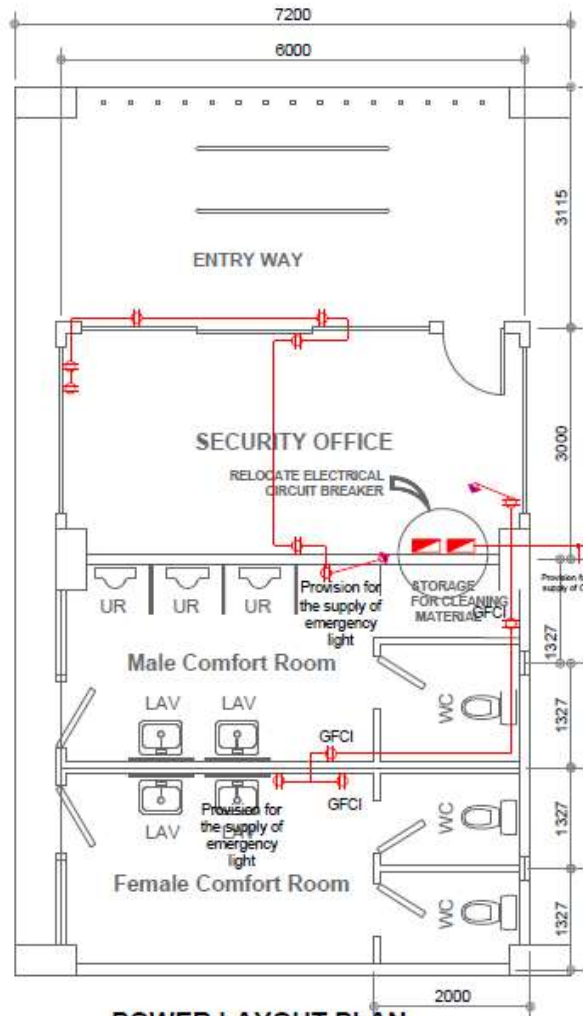
POWER LAYOUT PLAN
