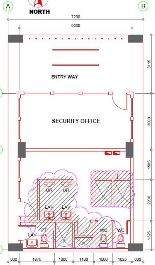
PREVIOUS LAYOUT PLAN
