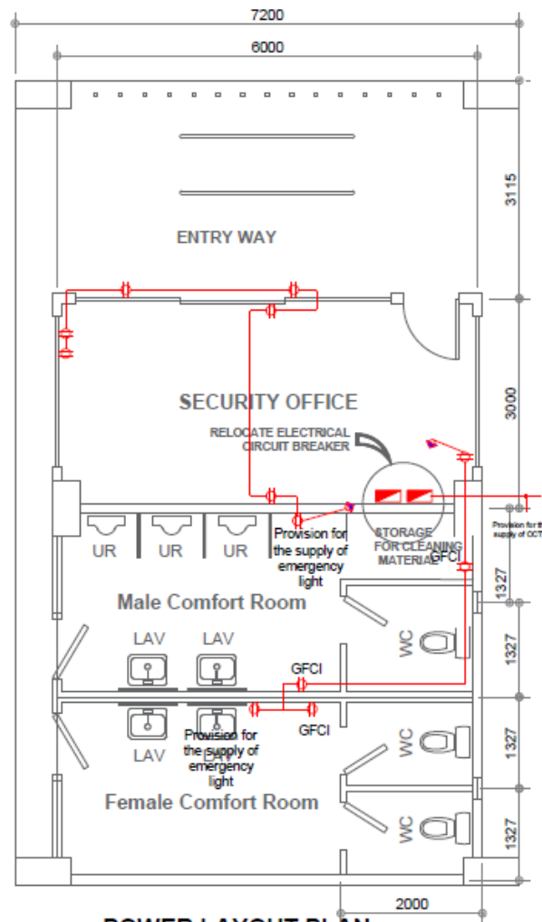
POWER LAYOUT PLAN
