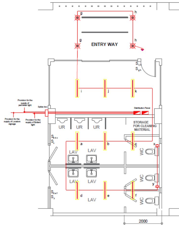
LIGHTING LAYOUT PLAN
