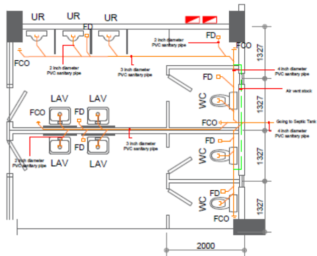
PROPOSE SEWER LINE LAYOUT PLAN
